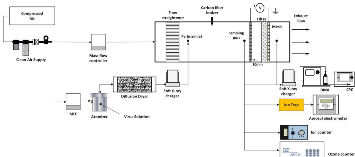
Fig. 1. Experimental setup.
